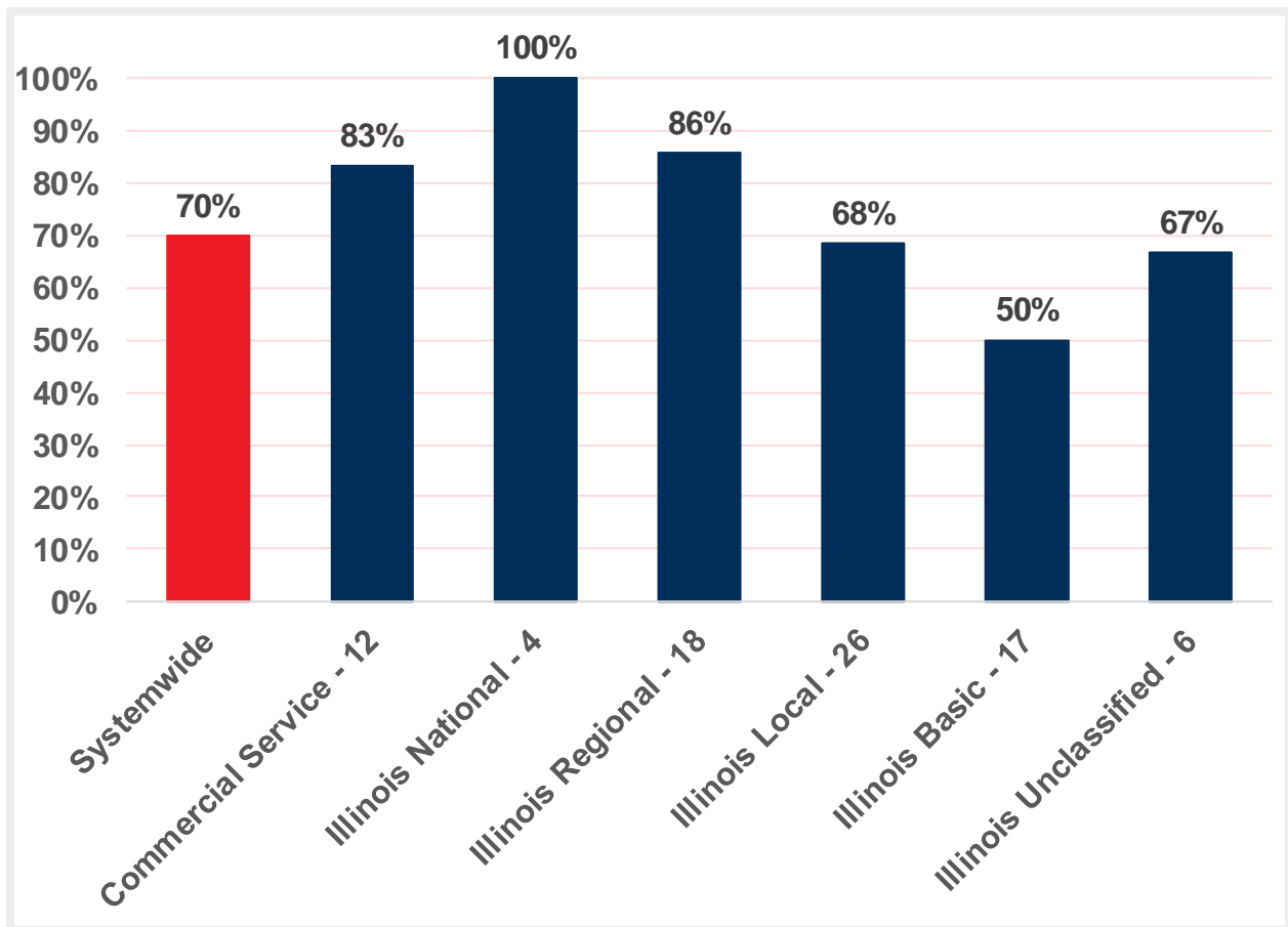
Figure 6.9. RPZ Analysis – Buildings or Structures
