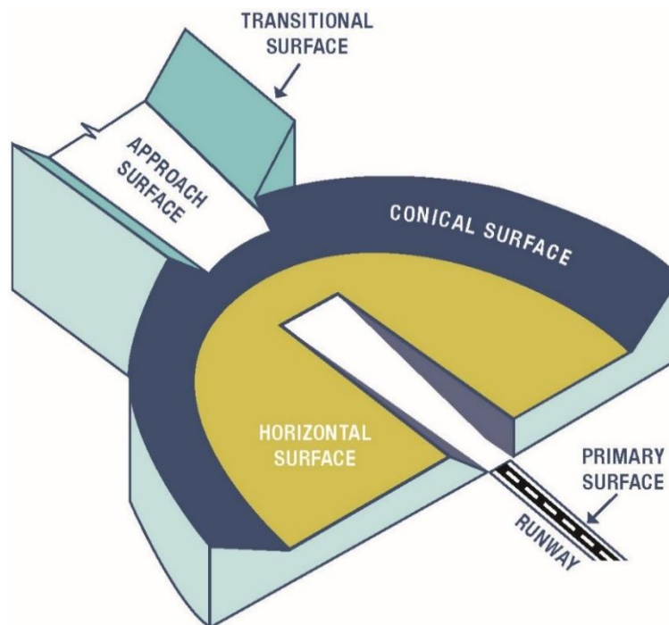
Figure 6.3. Part 77 Imaginary Surfaces
