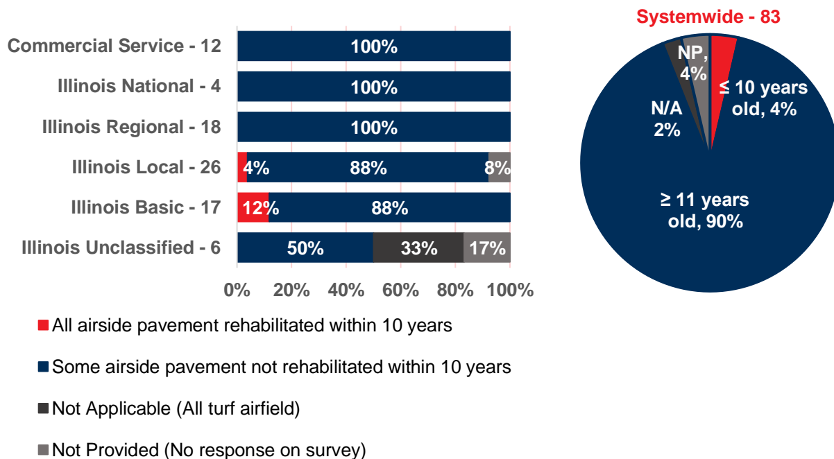
Figure 3.19. Percent of Airports with All Rehabilitated Airside Pavement Less Than 10 Years Old
