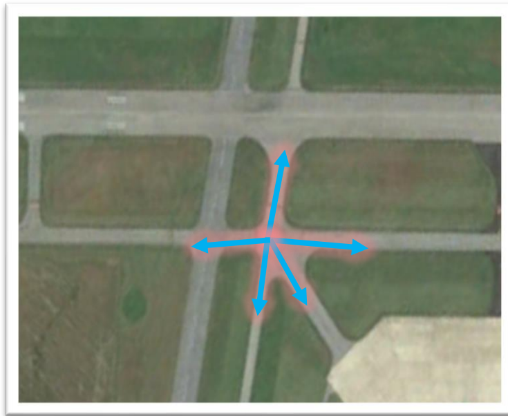
Figure 3.8. Three-Node Intersection
